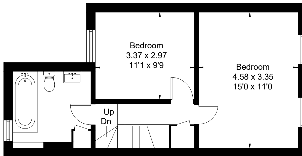
First Floor
